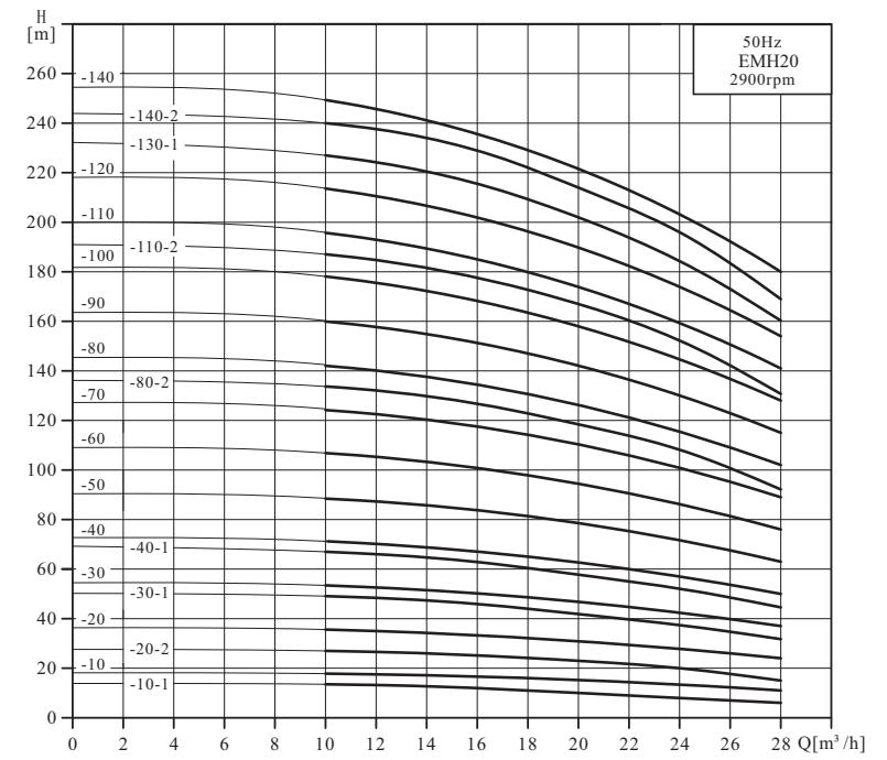
EMH20 Performance Curve
