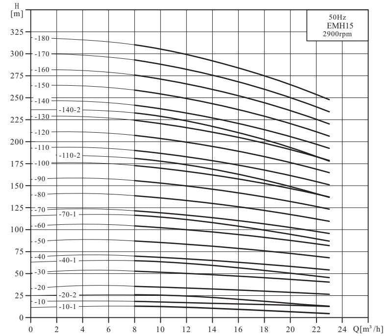
EMH15 Performance Curve
