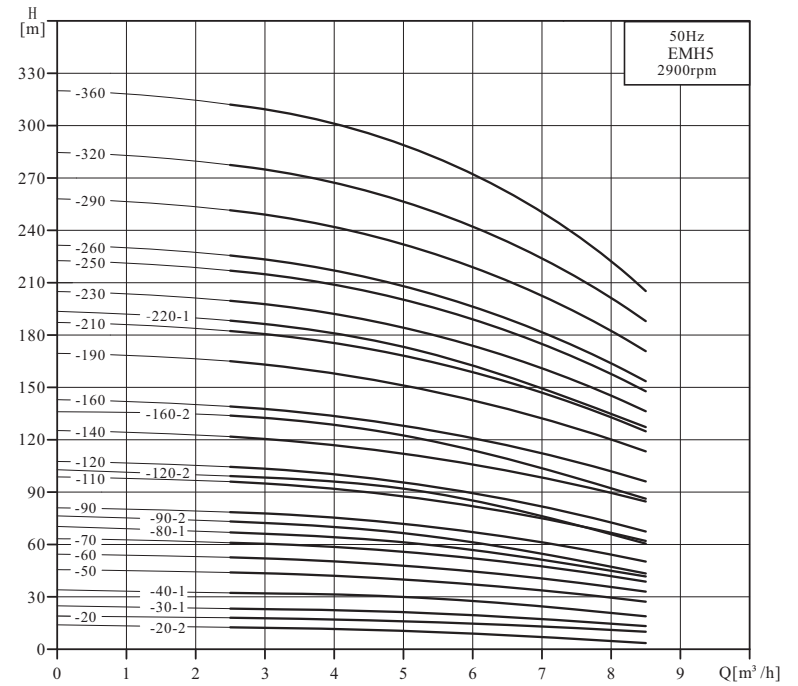
EMH5 Performance Curve
