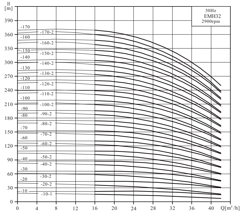
EMH32 Performance Curve
