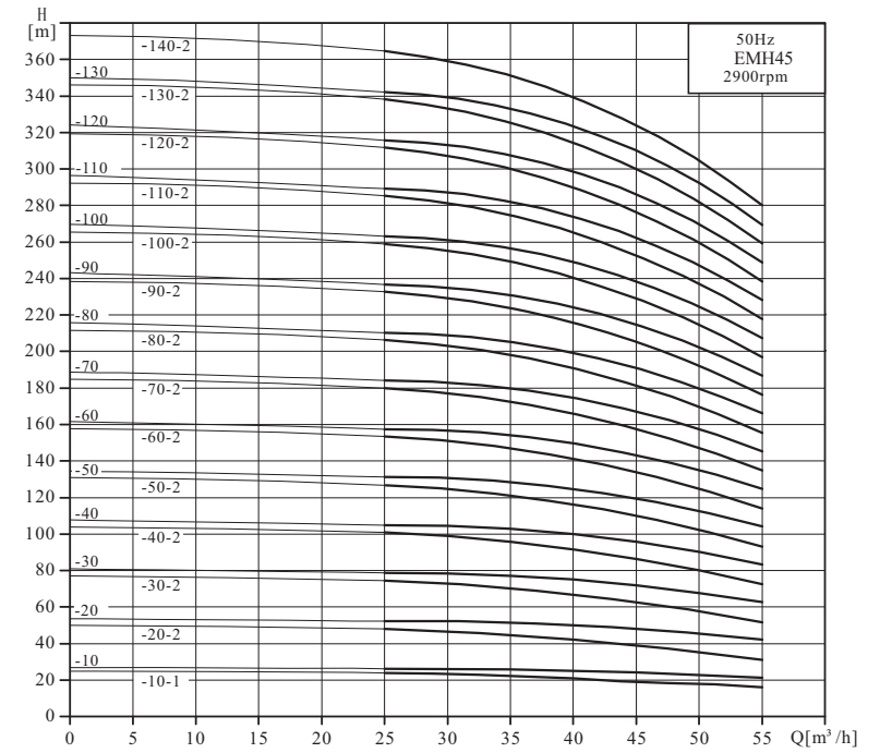
EMH45 Performance Curve
