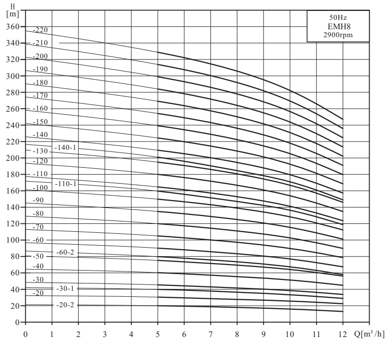
EMH8 Performance Curve
