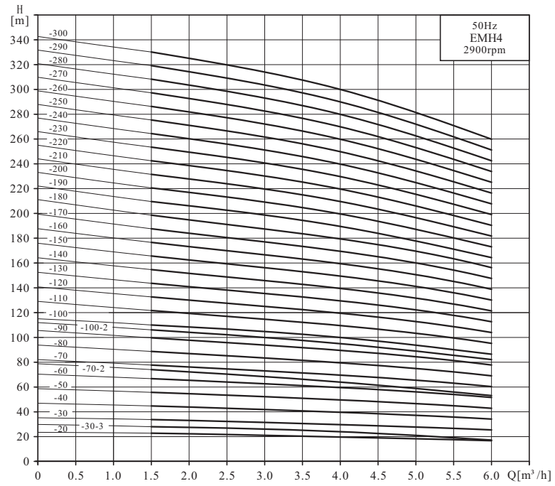
EMH4 Performance Curve
