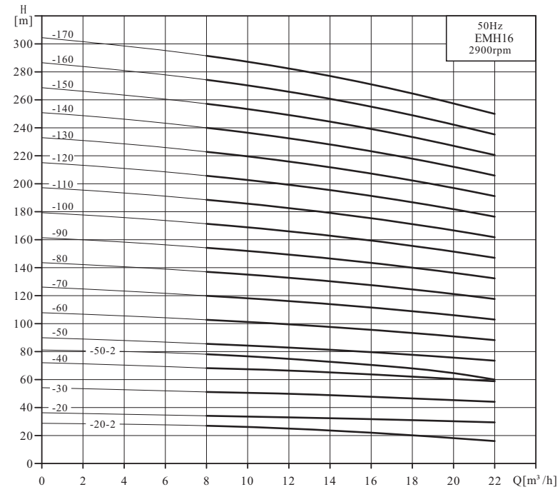
EMH16 Performance Curve
