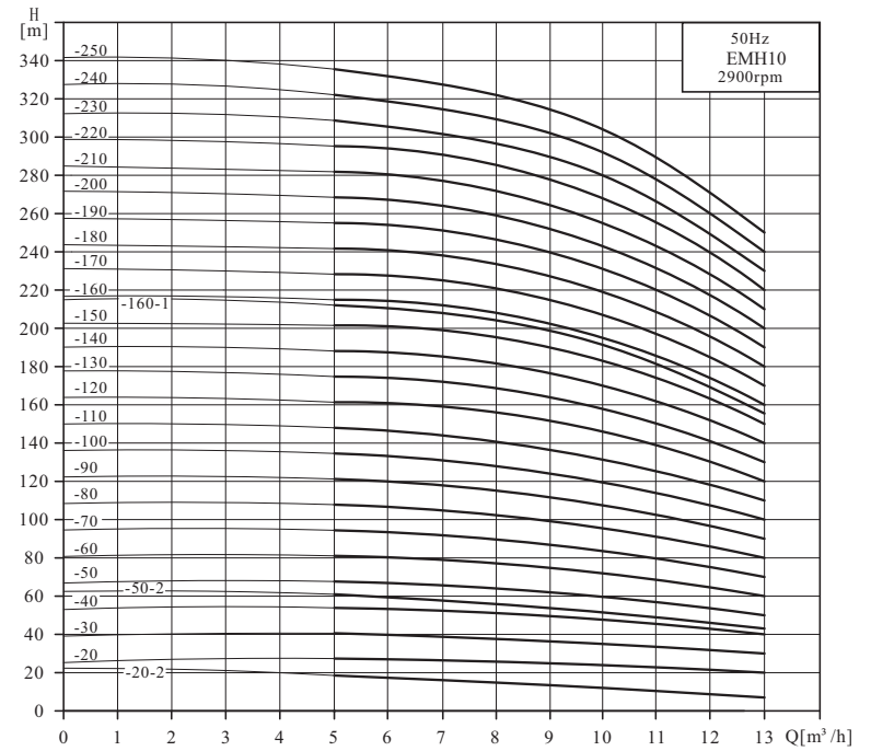
EMH10 Performance Curve
