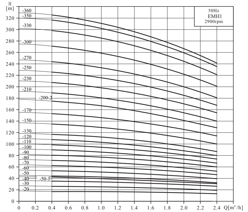
EMH1 Performance Curve
