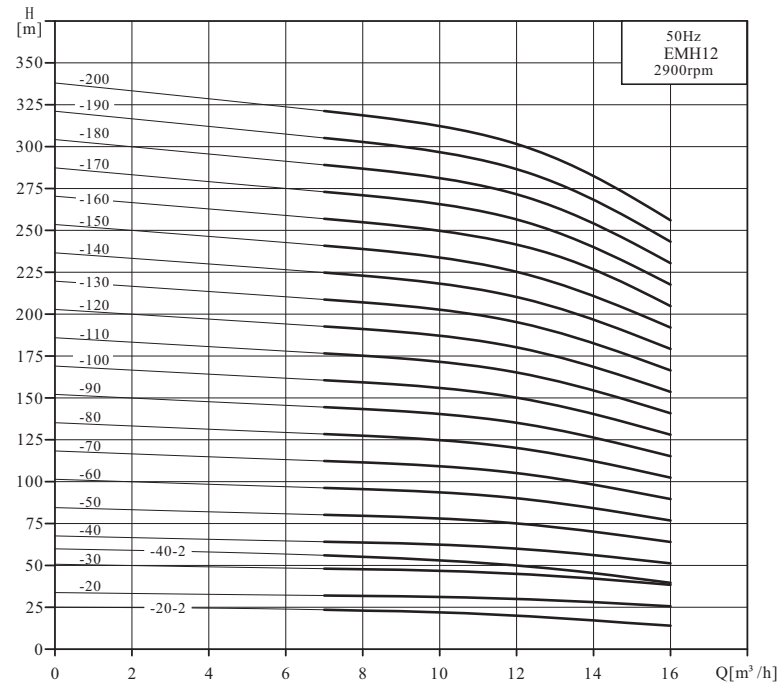
EMH12 Performance Curve
