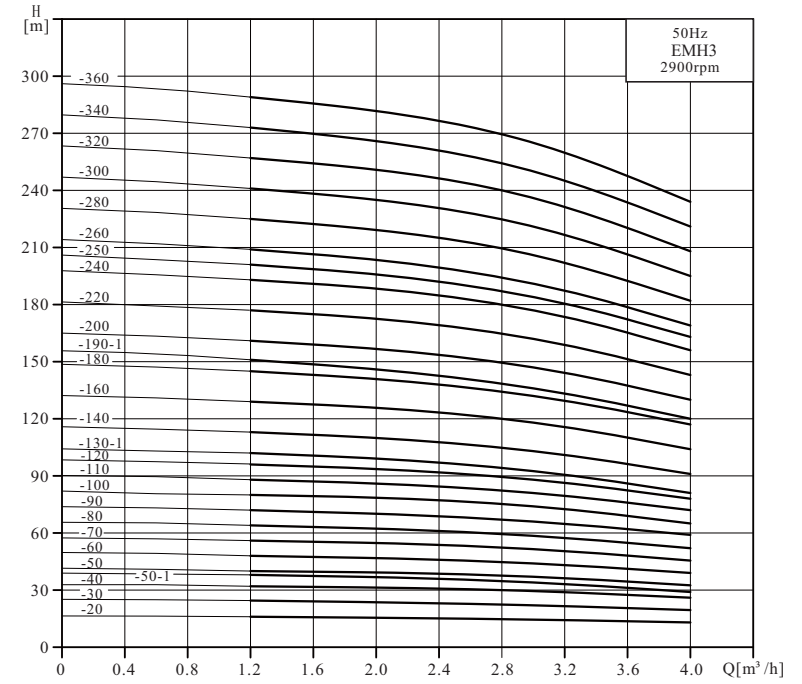
EMH3 Performance Curve
