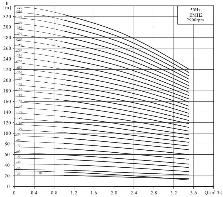
EMH2 Performance Curve
