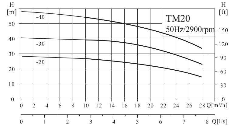
TM20 Performance Curve
