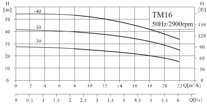
TM16 Performance Curve
